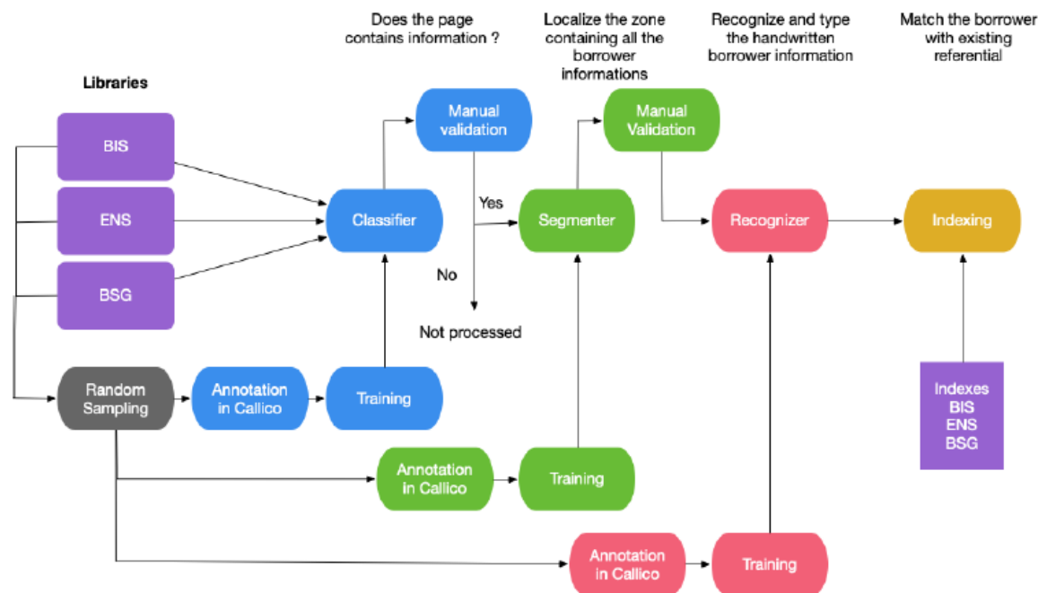
FIGURE 3 – The comprehensive workflow for automated document processing in the PRET19 project. It starts with the BIS, ENS and BSG library registers, where pages are first classified to determine whether they contain relevant borrower information. Pages identified as containing information undergo further processing, including segmentation and recognition stages, followed by indexing to match recognised borrower details with existing reference data. The workflow also includes a feedback loop to train the classifier and recogniser using annotations made in Callico based on randomly sampled data and manual corrections to improve accuracy and performance.
